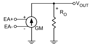
Figure 4. Equivalent circuit
