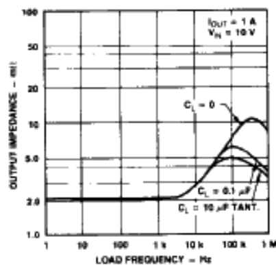
Output Impedance
