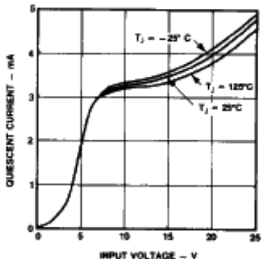
Quiescent Current
