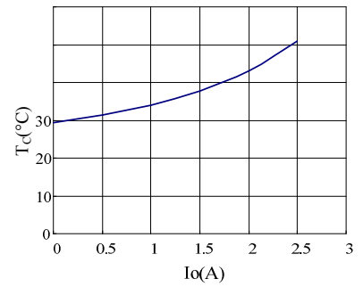
Case Temperature vs Output Current
