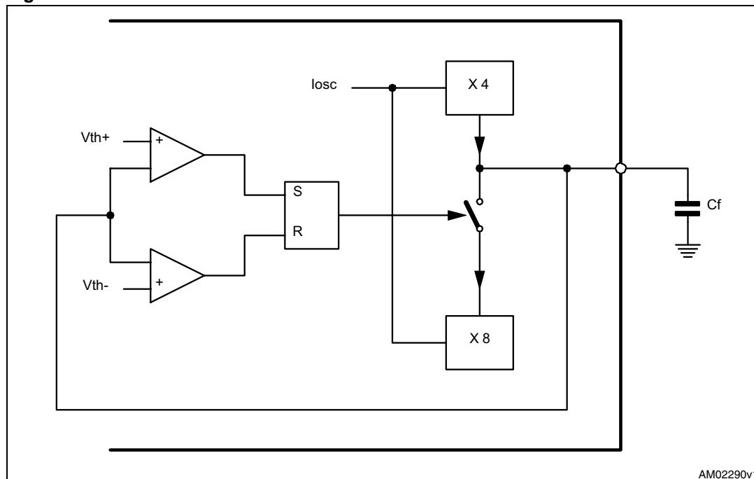
Figure 7. Oscillator block
