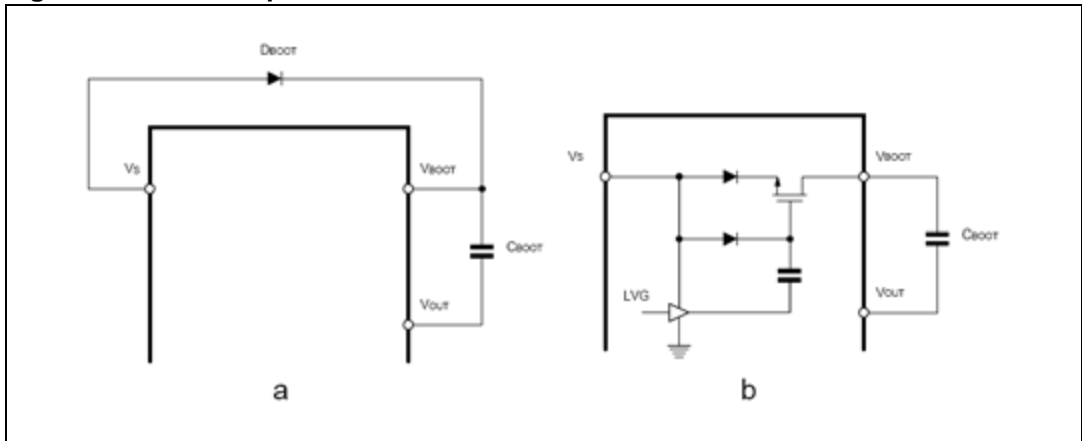
Figure 13. Bootstrap driver
