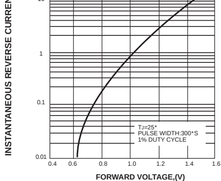
FIG. 4-TYPICAL FORWARD CHARACTERISTICS PER BRIDGE ELEMENT
