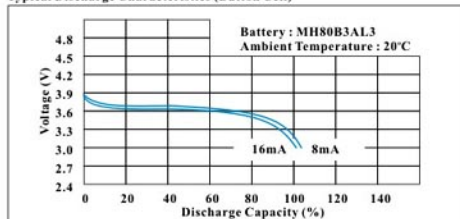
Typical Discharge Characteristics (Button Cell)
