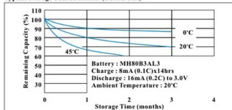
Typical Storage Characteristics (Button Cell)
