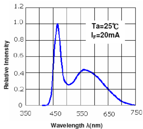
< Figure 4 Wavelength & relative intensity for PLCC 5050 series.>
