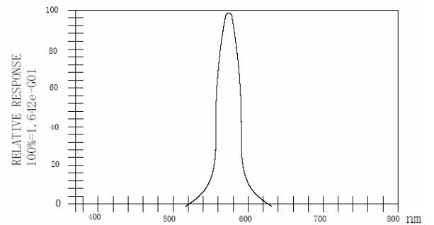
Luminous Spectrum (Ta=25°C)
