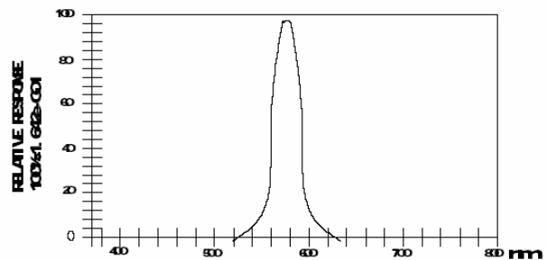
Luminous Spectrum ( T_a=25^\circ\text{C} ) SPECTRAL RADIANCE
