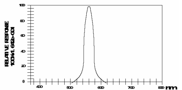
Luminous Spectrum ( T_a=25^\circ\text{C} ) SPECIAL PACKAGE
