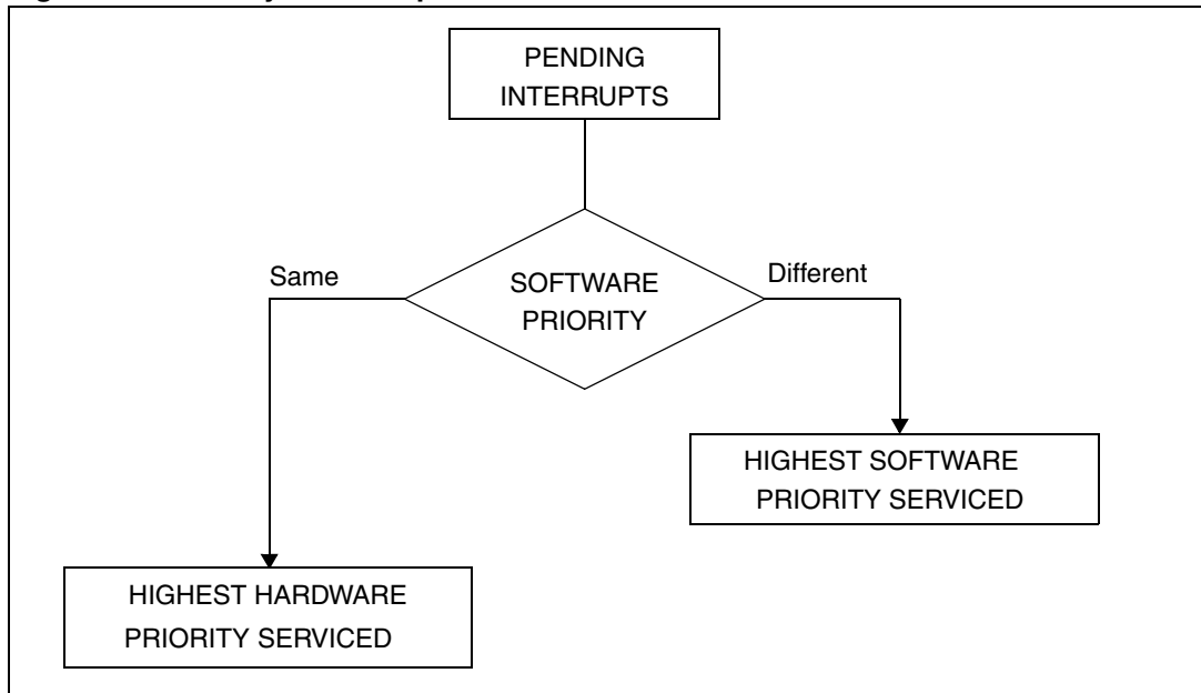
Figure 29. Priority decision process
