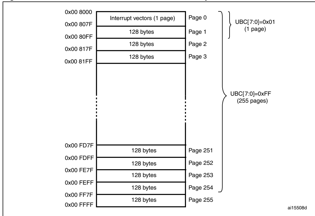
Figure 8. UBC area size definition for medium density devices
