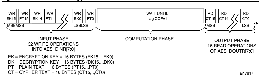
Figure 136. Mode 1: encryption
