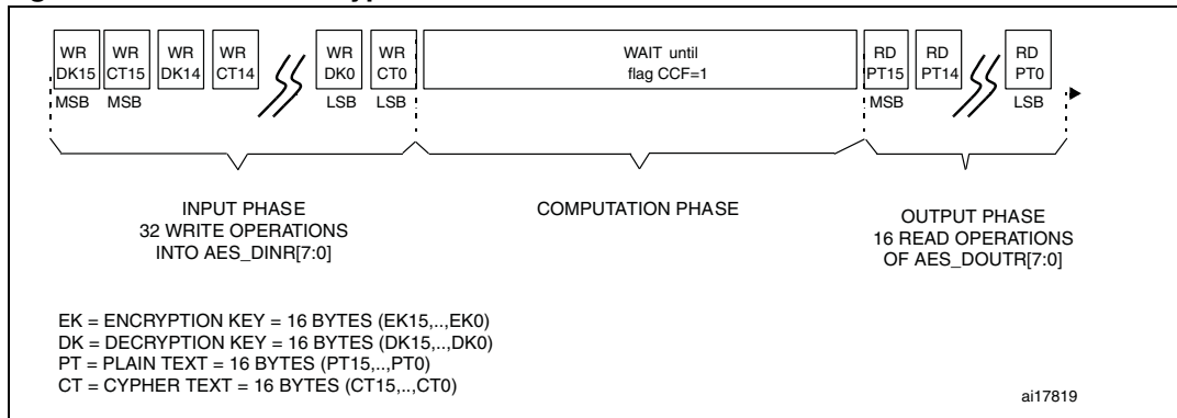
Figure 138. Mode 3: decryption
