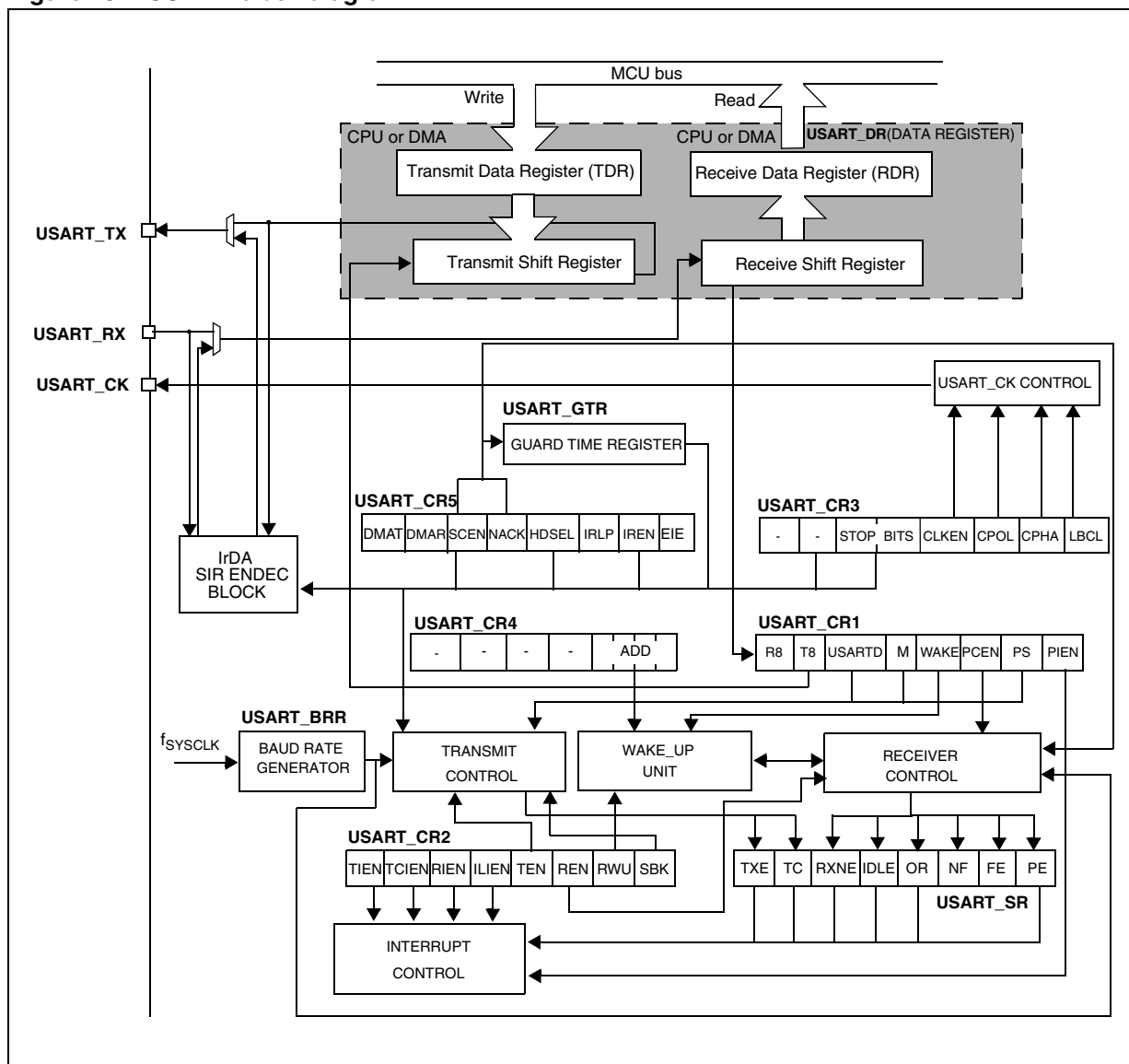
Figure 152. USART block diagram
