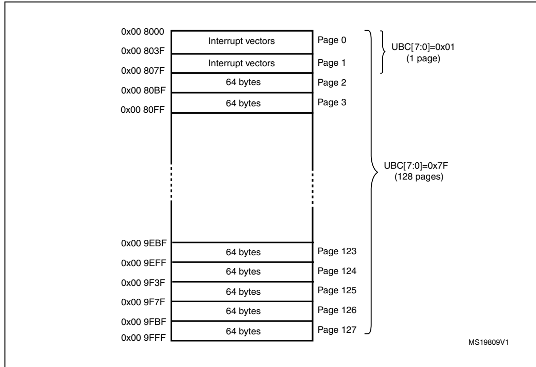
Figure 7. UBC area size definition for low density devices
