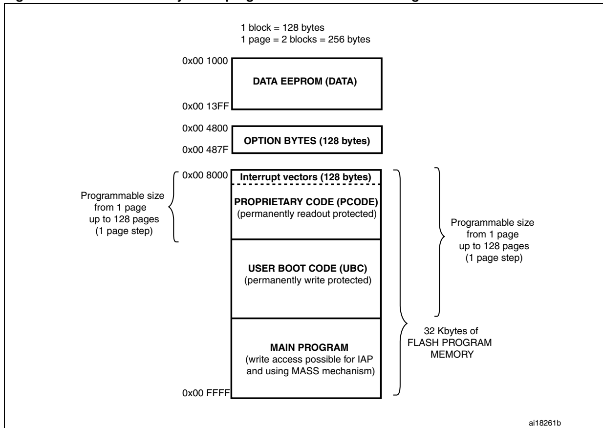
Figure 5. Medium+ density Flash program and data EEPROM organization
