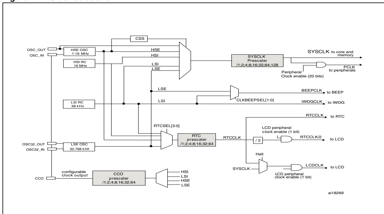
Figure 17. Clock structure
