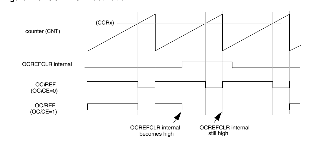
Figure 115. OCREFCLR activation
