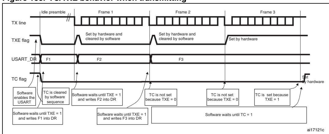
Figure 155. TC/TXE behavior when transmitting
