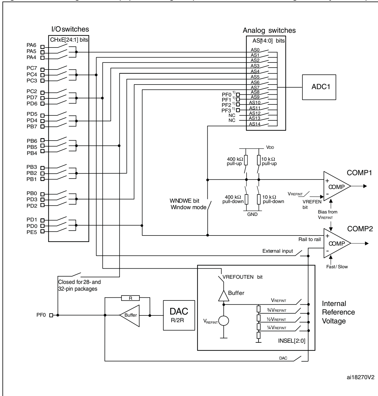
Figure 23. Routing interface (RI) block diagram (medium, medium+ and high density devices)
