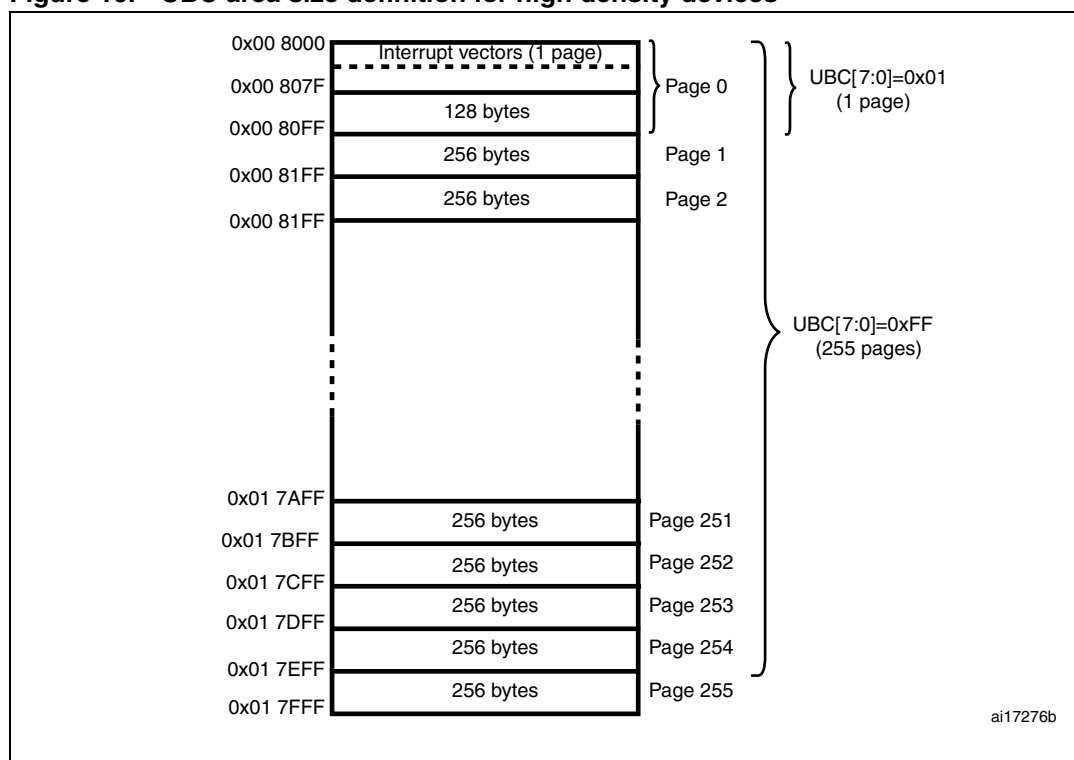
Figure 10. UBC area size definition for high density devices
