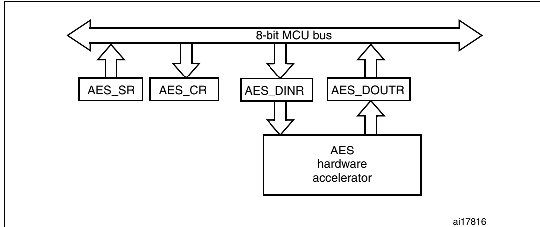
Figure 135. Block diagram
