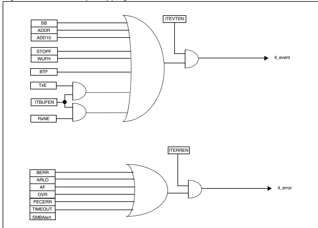
Figure 151. I 2 C interrupt mapping
