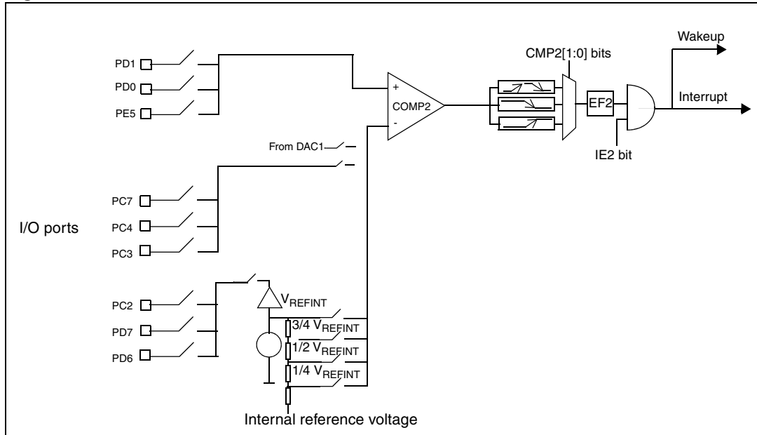
Figure 52. COMP2 interconnections
