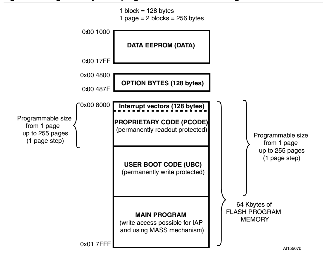
Figure 6. High density Flash program and data EEPROM organization
