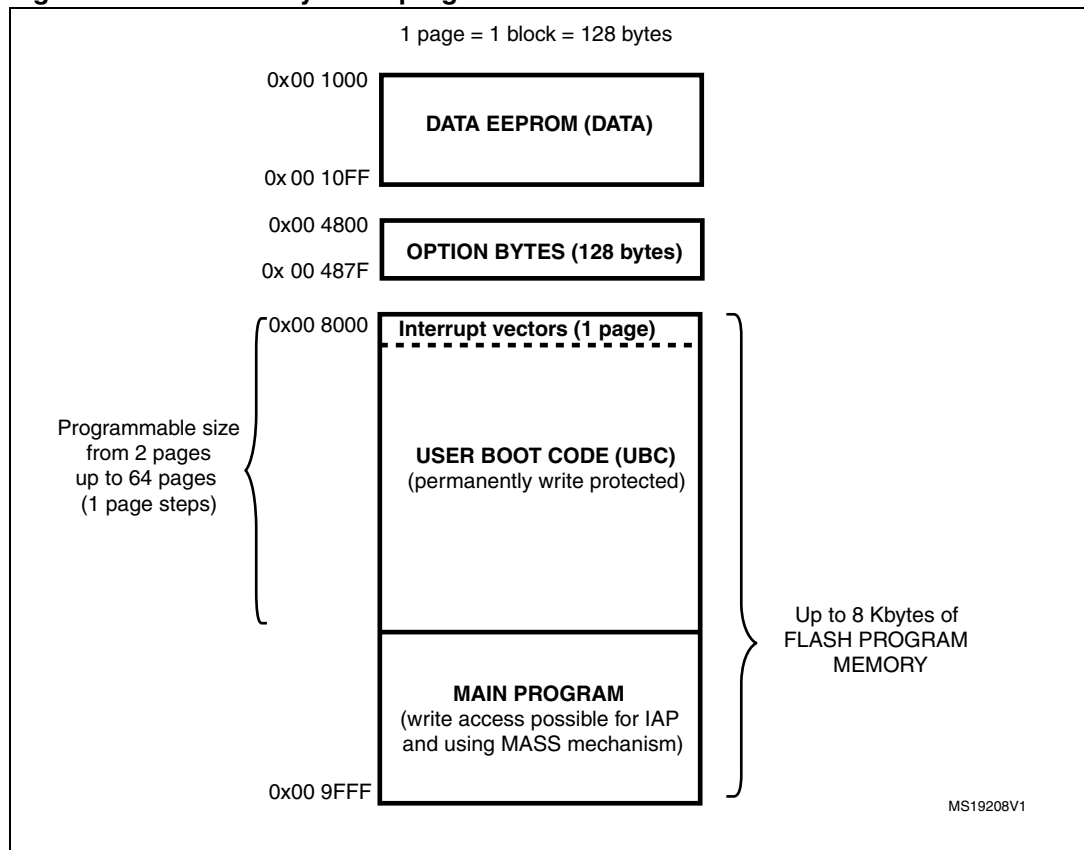
Figure 3. Low density Flash program and data EEPROM
