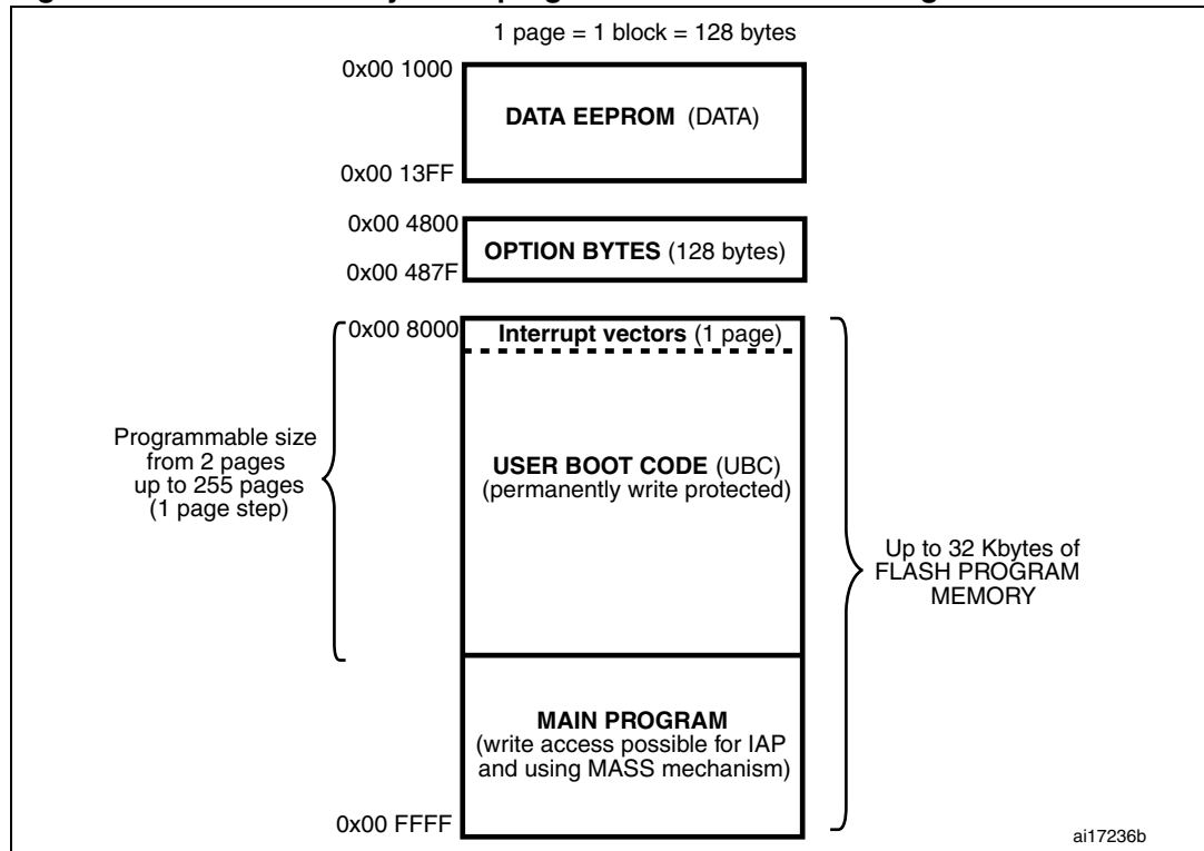
Figure 4. Medium density Flash program and data EEPROM organization
