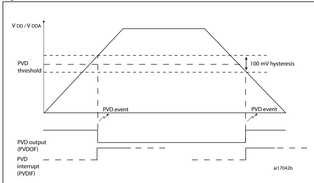
Figure 15. PVD threshold
