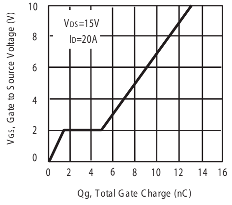
Figure 11. Gate Charge
