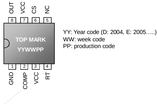
SOP-8 & DIP-8 (TOP VIEW)
