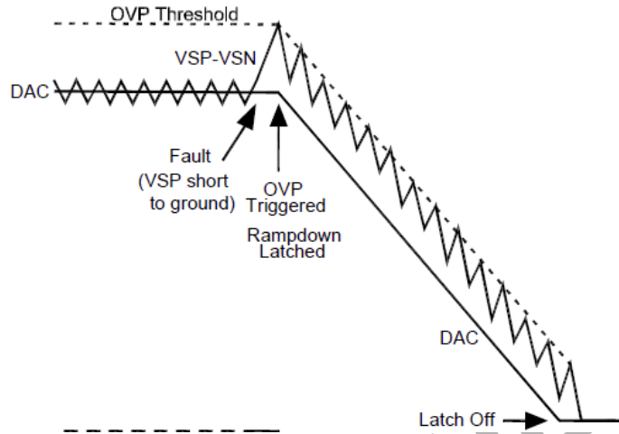
Figure 15. OVP During Normal Operation Mode
