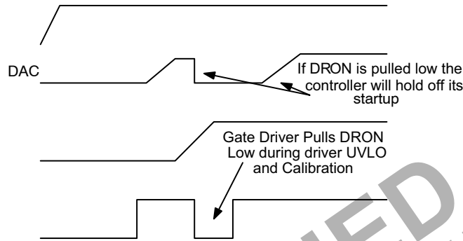
Figure 12. Gate Driver UVLO Restart
