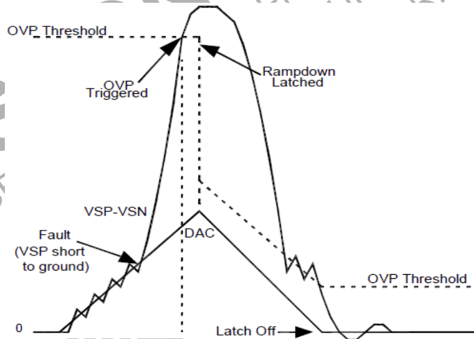
Figure 16. OVP Behavior at Startup
