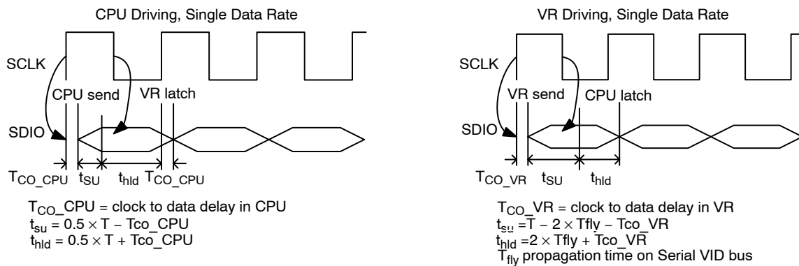
Figure 5. SVID Timing Diagram
