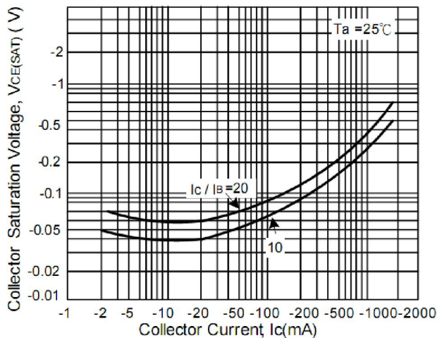
Figure 3. Collector-Emmitter Saturation Voltage
