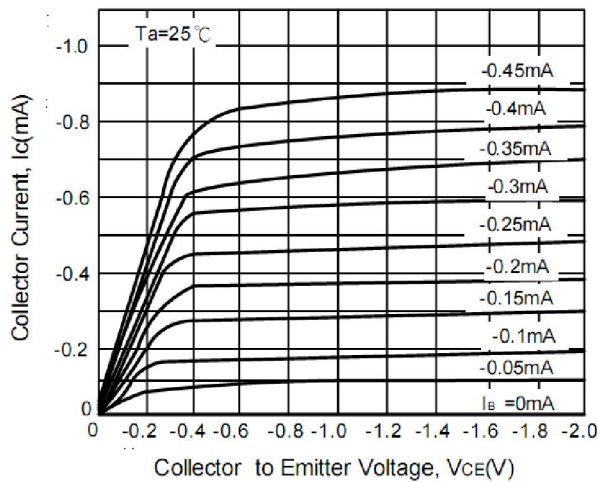
Figure 1. Static Characteristic
