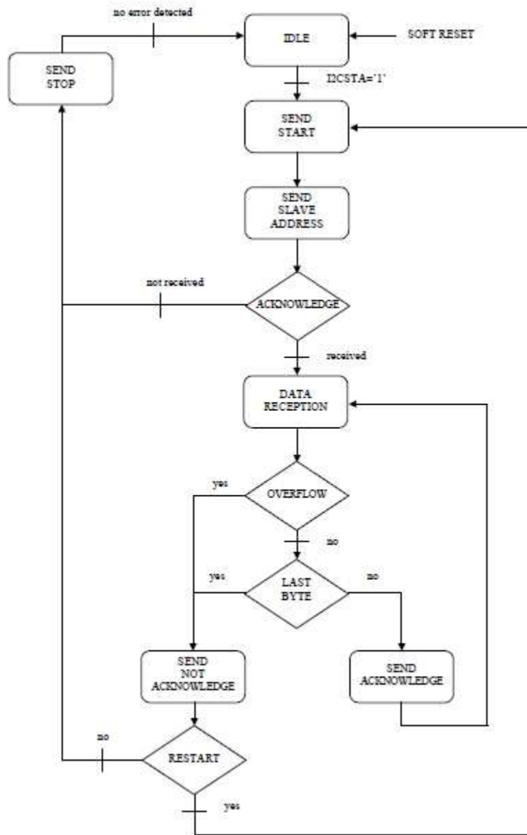
Figure 26 Reception FSM
