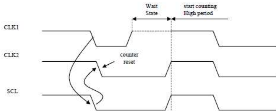
Figure 20 Clock synchronization
