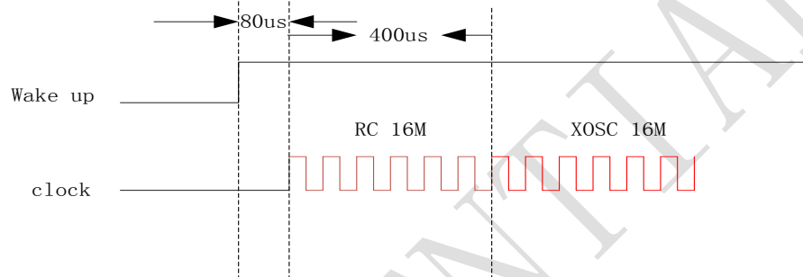
Figure 8 wake up process
