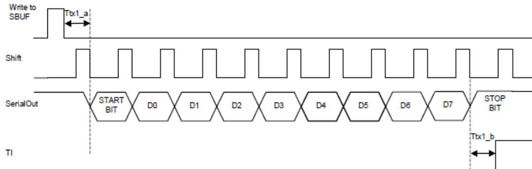
Figure 10 Serial Transmit Mode 1
