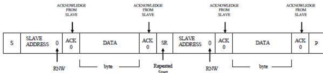
Figure 22 Repeated Start or Stop condition after last byte
