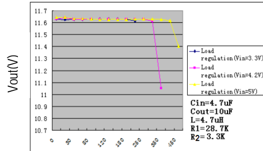
Load regulation
