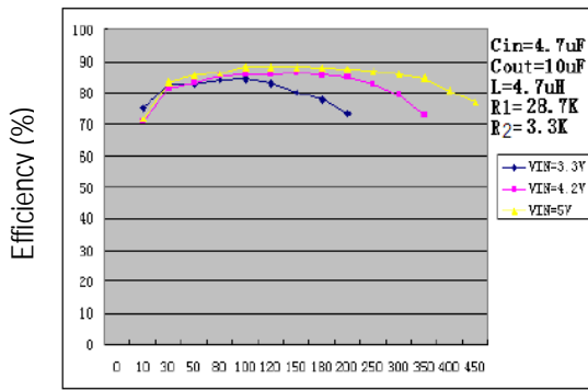
Efficiency Curve
