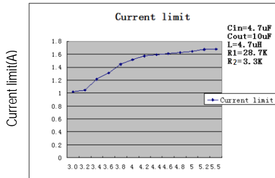
Current limit vs. Vin
